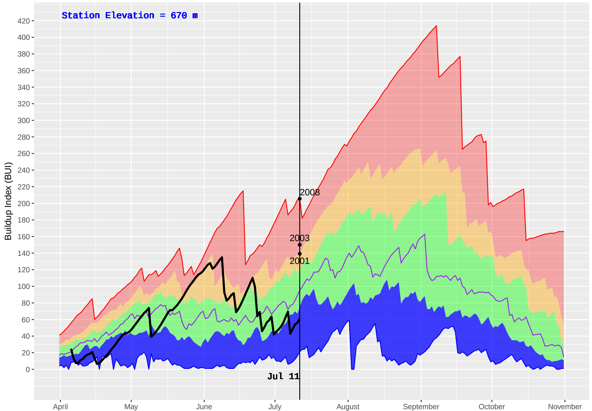
FINTRY (298) : Historical (1989–2016) and Current (2018) Noon Buildup Index (BUI)
